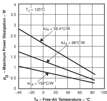
Figure 8-13. Maximum Power Dissipation vs Ambient Temperature
