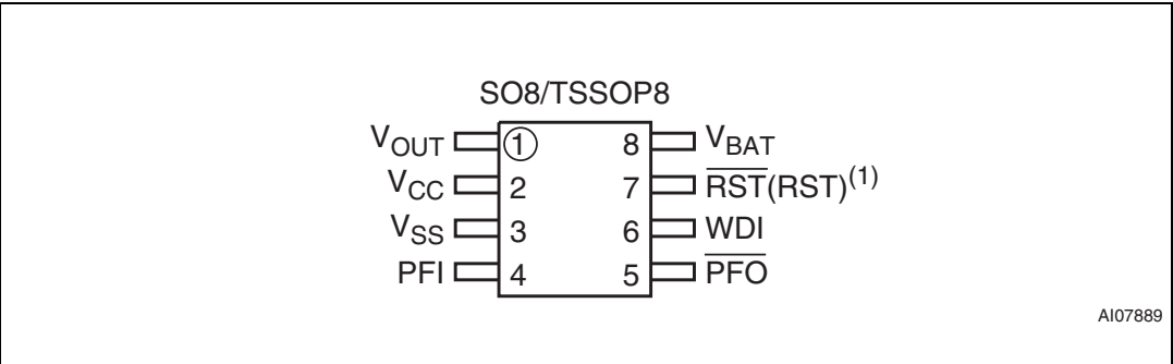
Figure 4. STM690A/692A/802/805/817 connections
