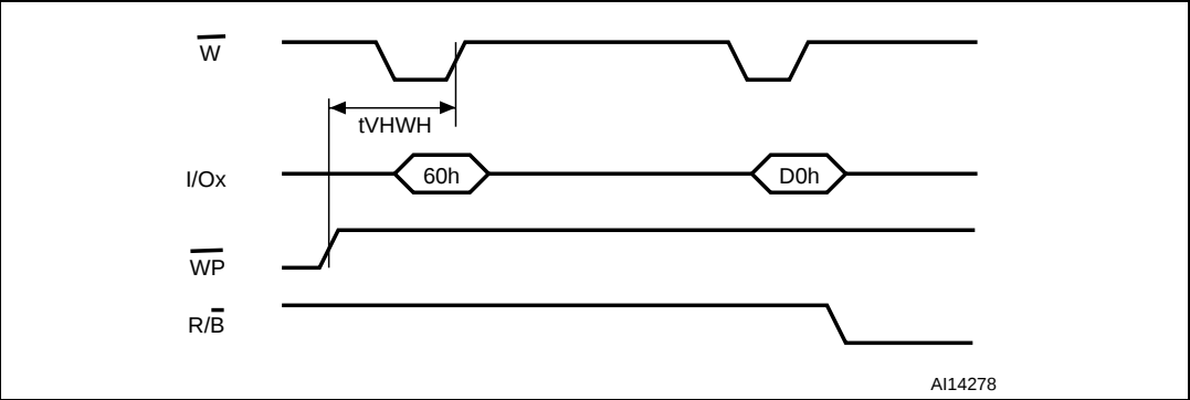
Figure 32. Erase enable waveform
