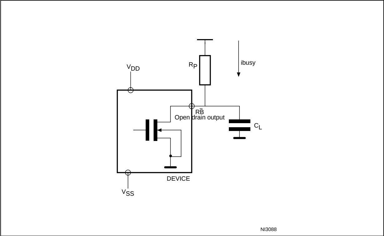
Figure 45. Ready/Busy load circuit
