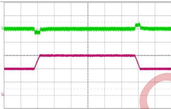
Figure 11. Output voltage response to load current step change (10A - 15A - 10A) at V_{in} = 48 V . Top trace: output voltage (50mV/div.) Bottom: load current (5 A/div.). Current slew rate: 0.1 A/ \mu s. Time scale: 200 \mu s /div. C_o = 10\mu F tantalum + 1 \mu F ceramic
