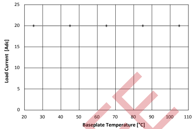
Figure 4. Coldplate cooling: Power derating of SQL48T20033-xxxxBx converter with baseplate option and coldplate cooling. No thermal derating required. (Conditions: Air velocity \leq 30\text{LFM} ( \leq 0.15\text{m/s} ), V_{in} = 48\text{ V} , T_B \leq 105^\circ\text{C} )
