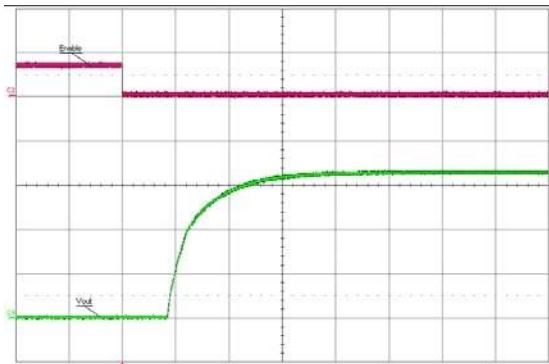
Figure 9. Turn-on waveform at full rated load current (resistive) with 10,000 uF output capacitor at V_{in}=48V , triggered via ON/OFF pin. Top trace: ON/OFF signal (5V/div.). Bottom trace: Output voltage (1V/div.). Time scale: 2 ms/div.
