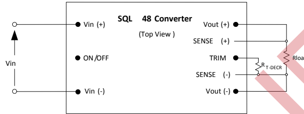
Figure D. Configuration for decreasing output voltage.
