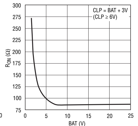
FBDIV R_{ON} vs \text{BAT}
