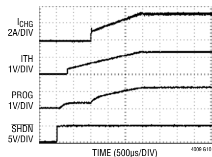
PWM Soft-Start
