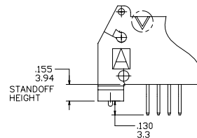
TERMINAL TYPE 3
