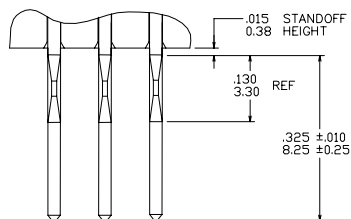
TERMINAL TYPE 2
