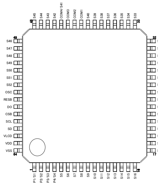
Fig.14 Pin Arrangement (BU97500KV)
