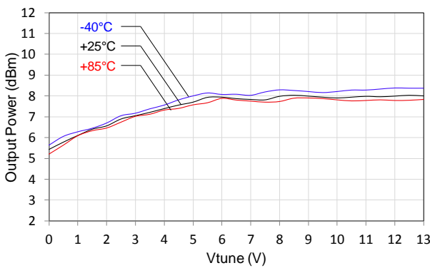
RFout/2 Output Power vs Tuning Voltage Vcc = 5V
