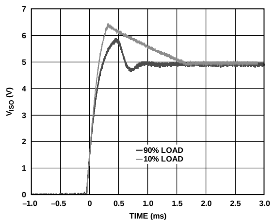
Figure 21. Typical Output Voltage Start-Up Transient at 10% and 90% Load, V_{ISO} = 5\text{ V}
