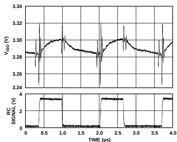
Figure 20. Typical Output Voltage Ripple at 90% Load, V_{ISO} = 3.3\text{ V}
