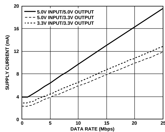
Figure 24. Typical I_{CHN} Supply Current per Reverse Data Channel (15 pF Output Load)
