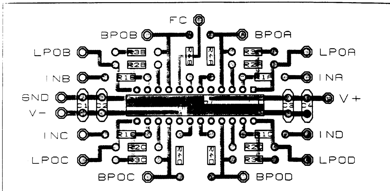
Figure 7a. MAX274 Suggested PC-Board Layout for DIP
