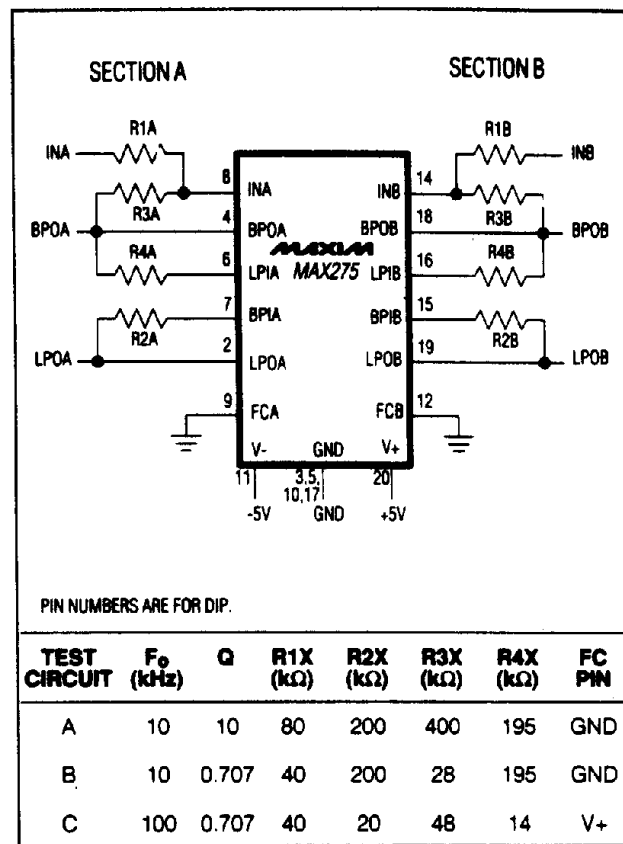
Figure 1b. MAX275 Connection Diagram and Test Circuit
