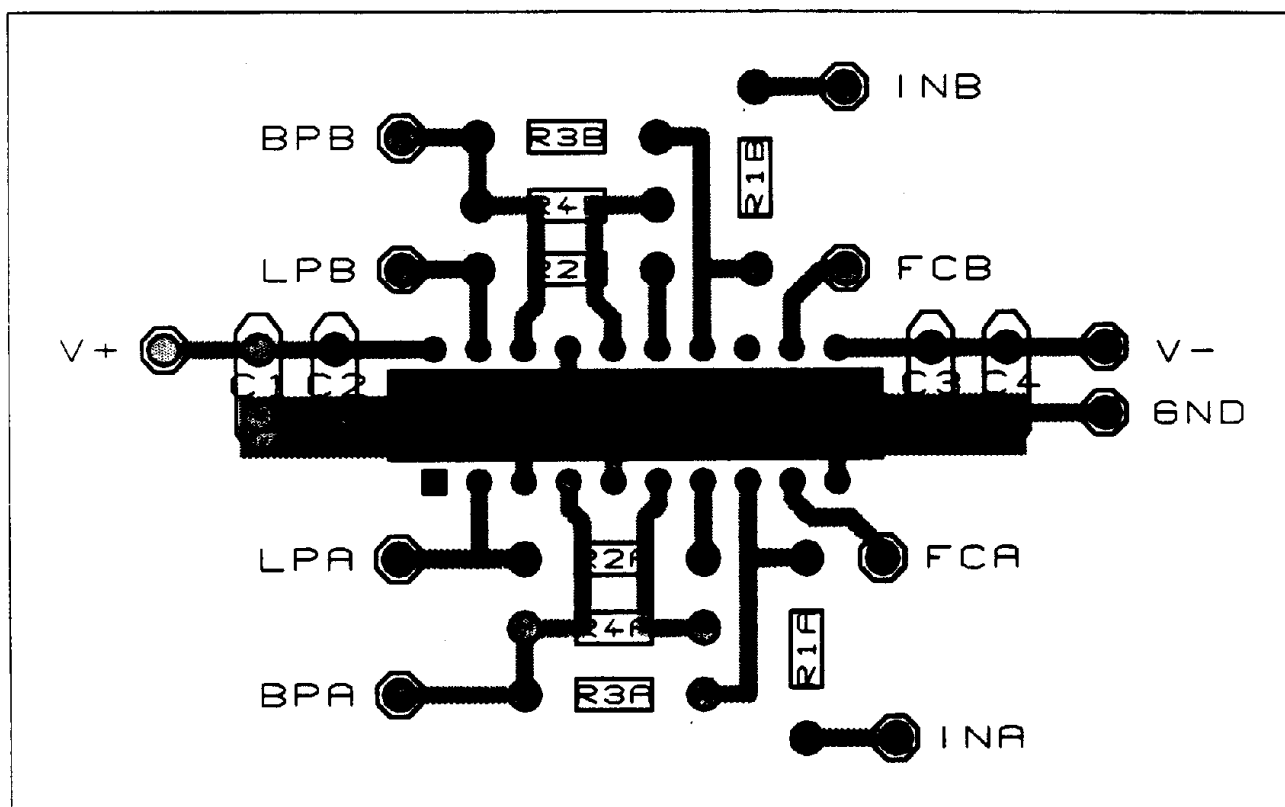
Figure 7b. MAX275 Suggested PC-Board Layout for DIP
