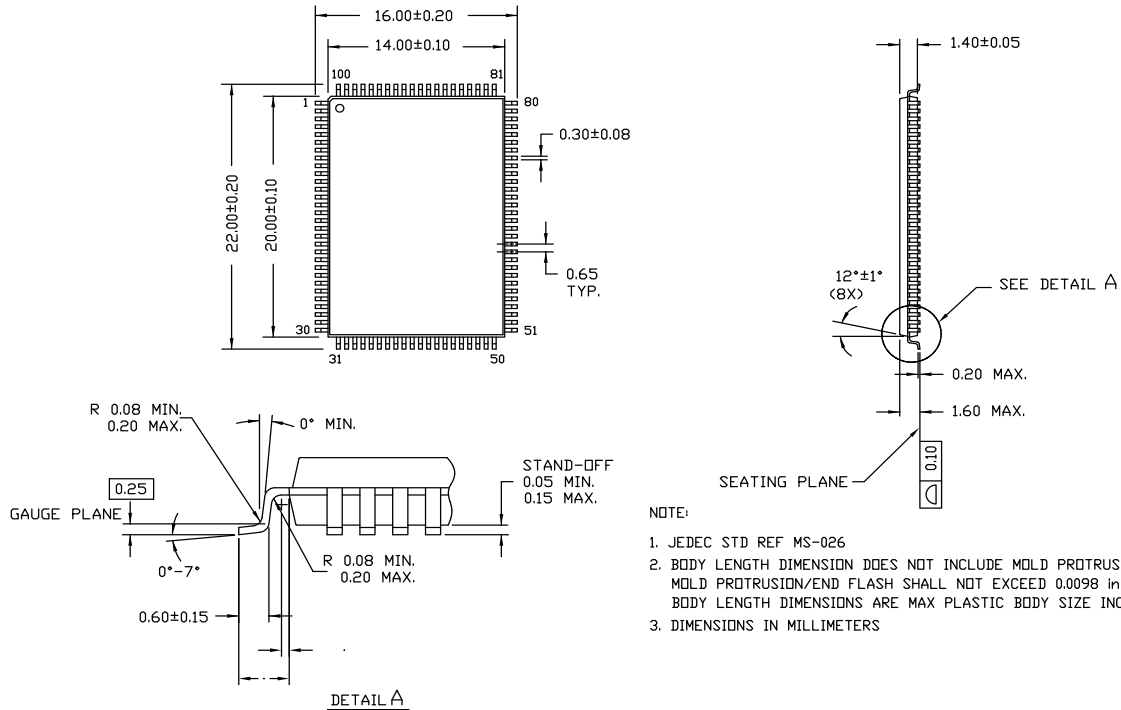
Figure 9. 100-pin TQFP (14 × 20 × 1.4 mm) A100RA Package Outline, 51-85050
