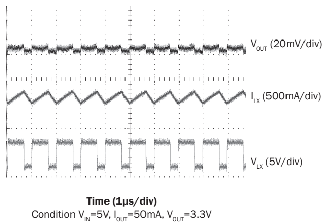
PWM Operation
