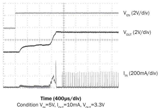
PSAVE Start-UP
