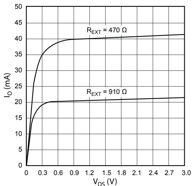
Channel Output Current versus Output Voltage
