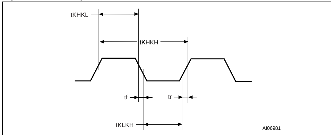
Figure 14. Clock input AC waveform
