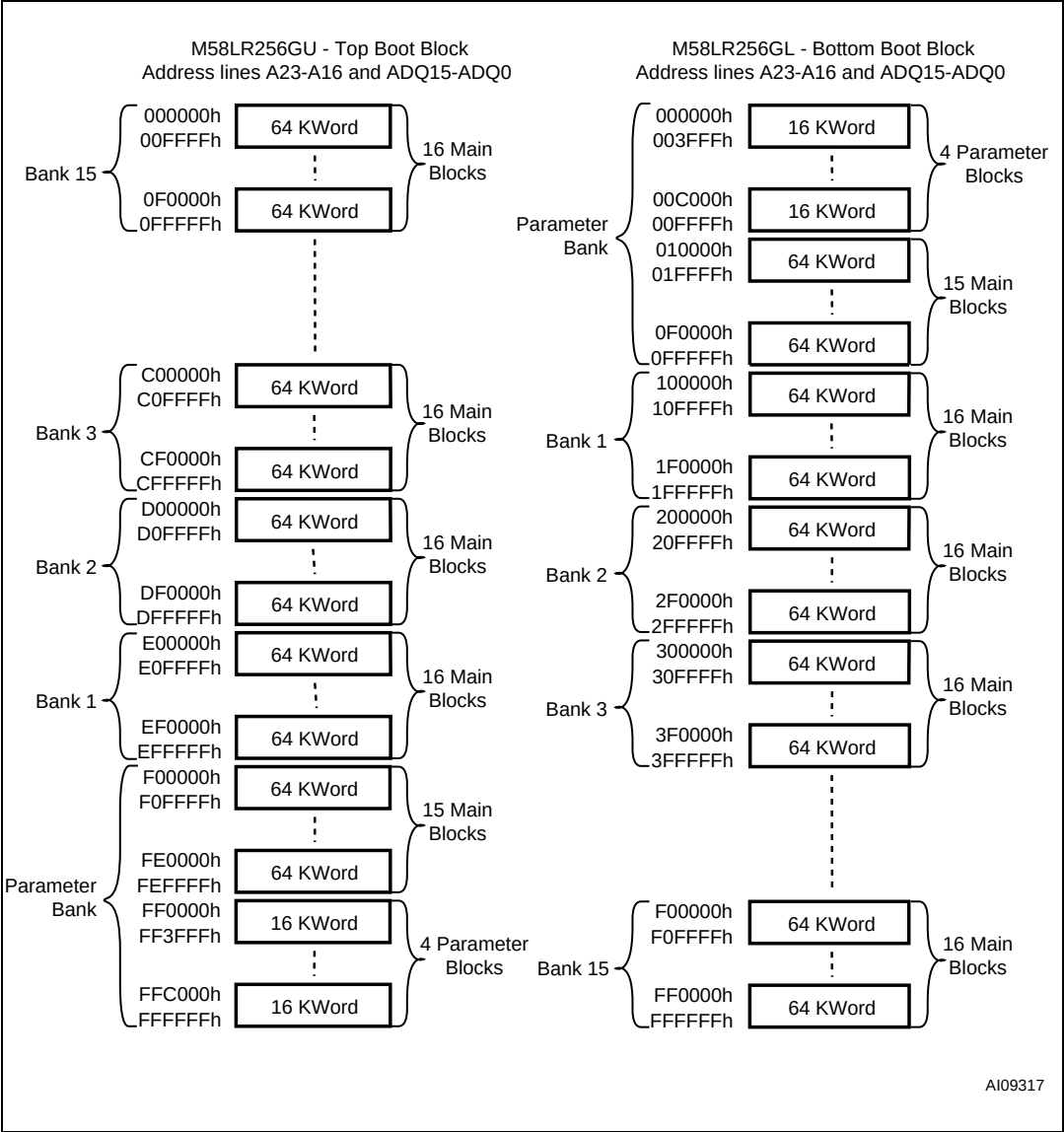
Figure 3. M58LR256GU/L memory map
