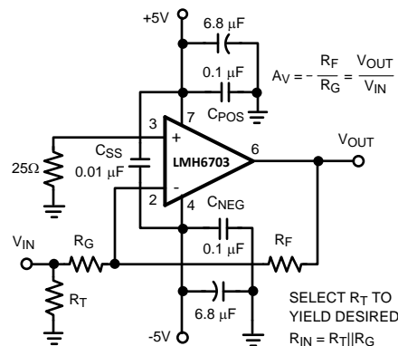
Figure 30. Recommended Inverting Gain Circuit (SOIC Pinout Shown)
