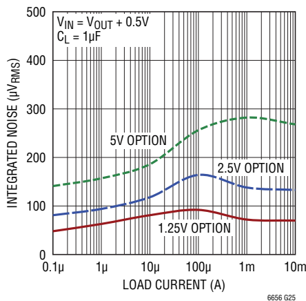
Integrated 10Hz to 1kHz Noise vs Load Current
