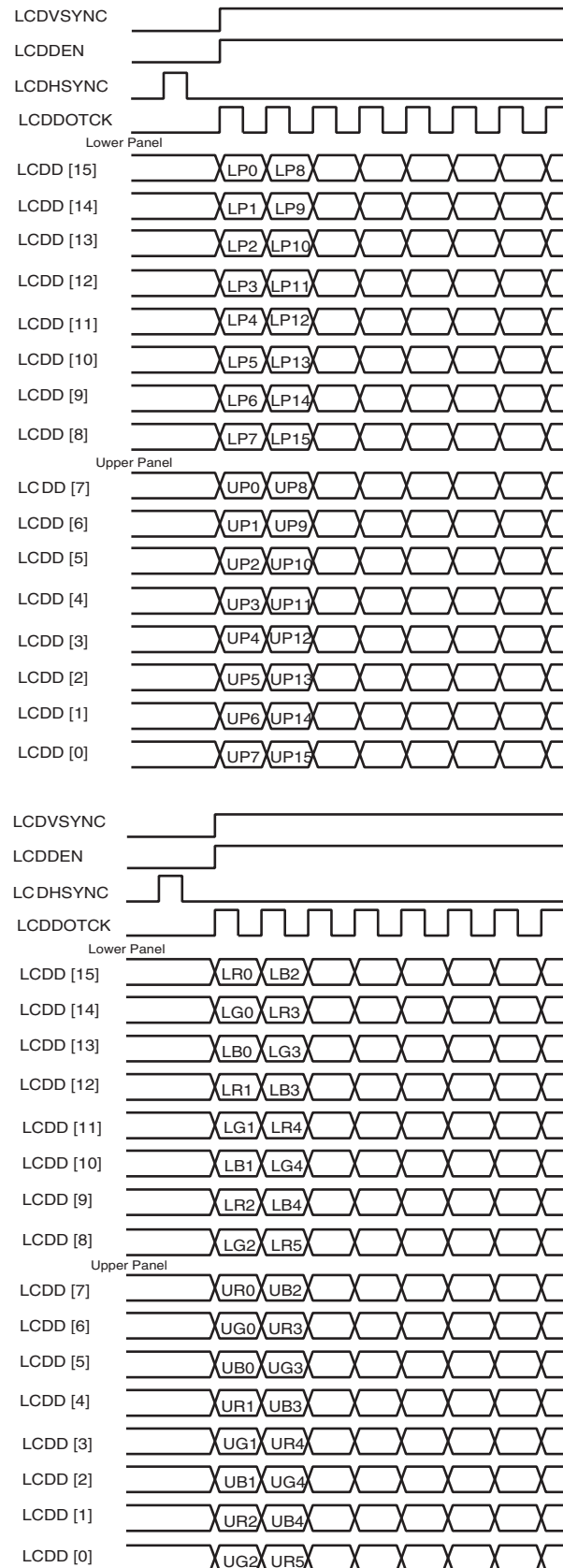
Figure 45-12. Dual Scan Monochrome and Color 16-bit Panel Timing (First Line Expanded View)
