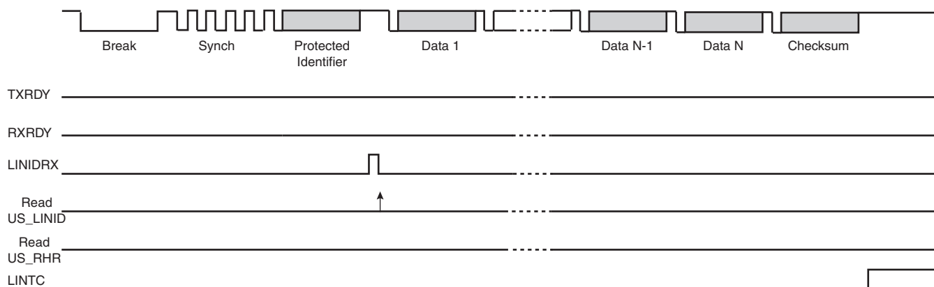
Figure 31-51. Slave Node Configuration, NACT = IGNORE
