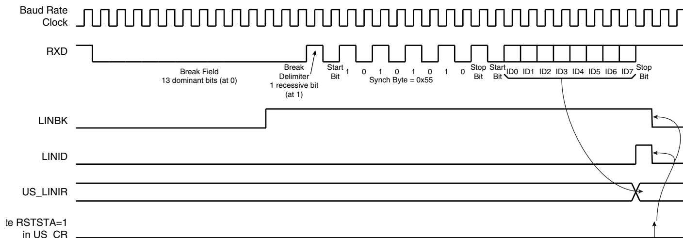
Figure 31-41. Header Reception
