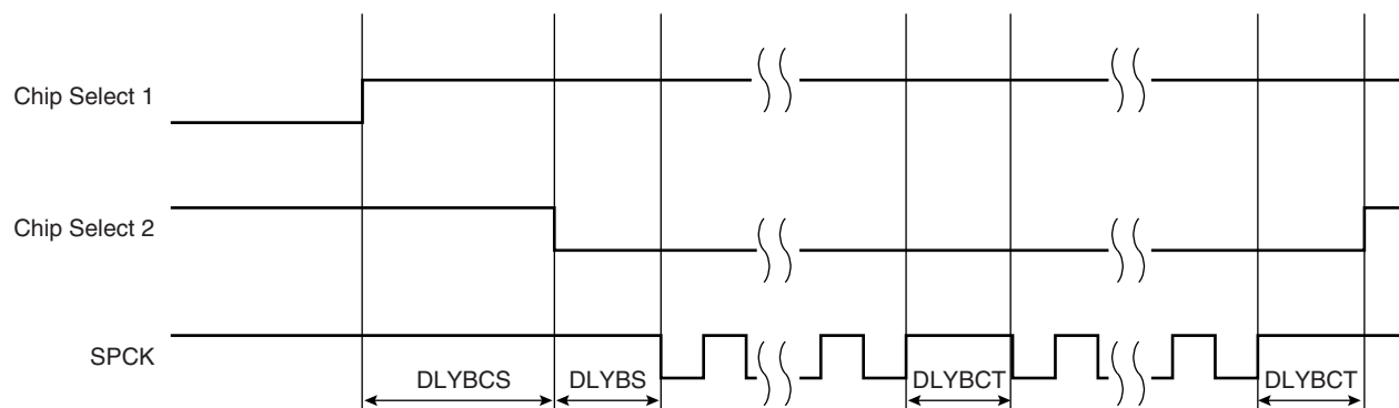
Figure 28-10. Programmable Delays
