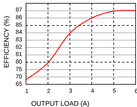
FEC30-24S3P3W Efficiency VS Output load
