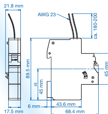
Dimensions UA120UL
