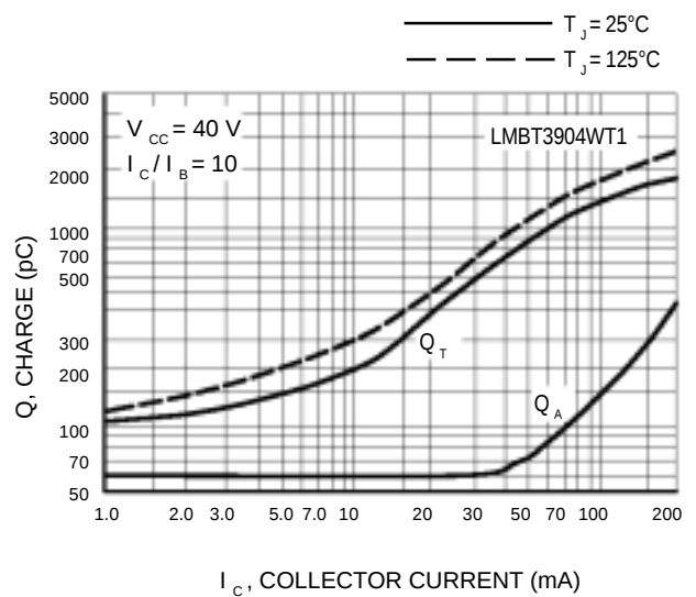
Figure 4. Charge Data
