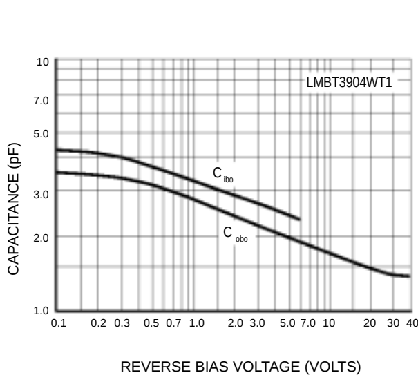
Figure 3. Capacitance
