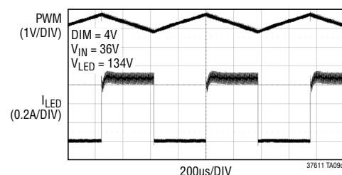
Dimming Waveform
