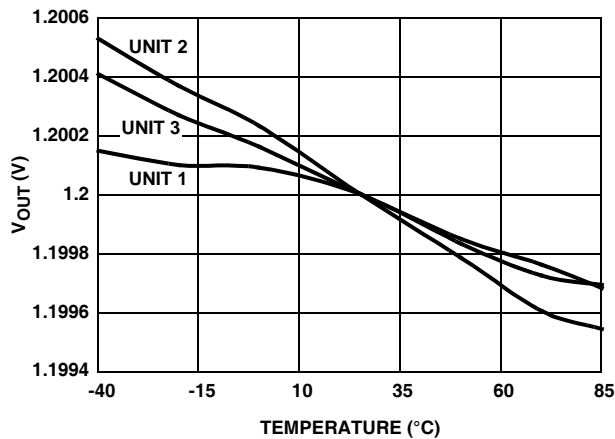
FIGURE 16. V_{OUT} vs TEMPERATURE NORMALIZED to +25°C
