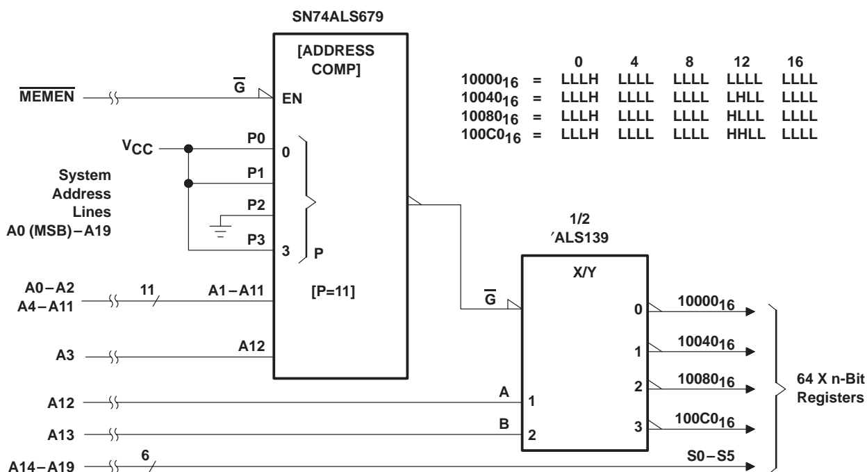
Figure 1. Register-Bank Decoder
