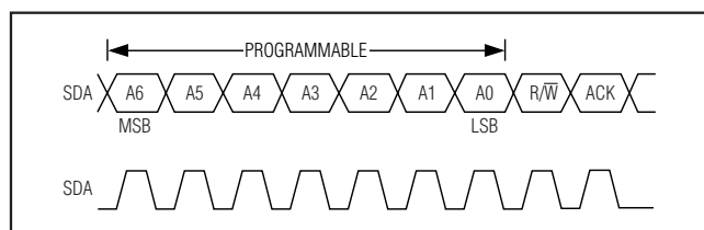
Figure 6. Slave Address
