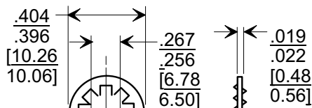
LOCK WASHER
