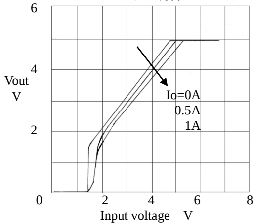
(2) Input voltage vs. Output voltage V_{IN}-V_{out}
