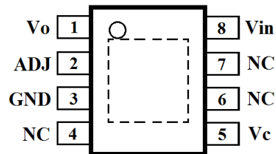
Pin Assign
