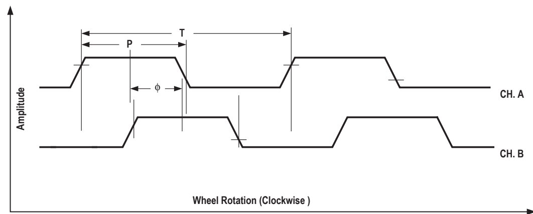
Figure 2. Output Waveform
