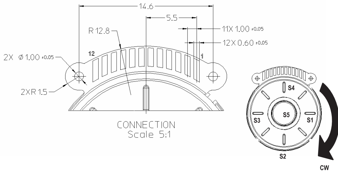
Figure 4. Electrical Connections
