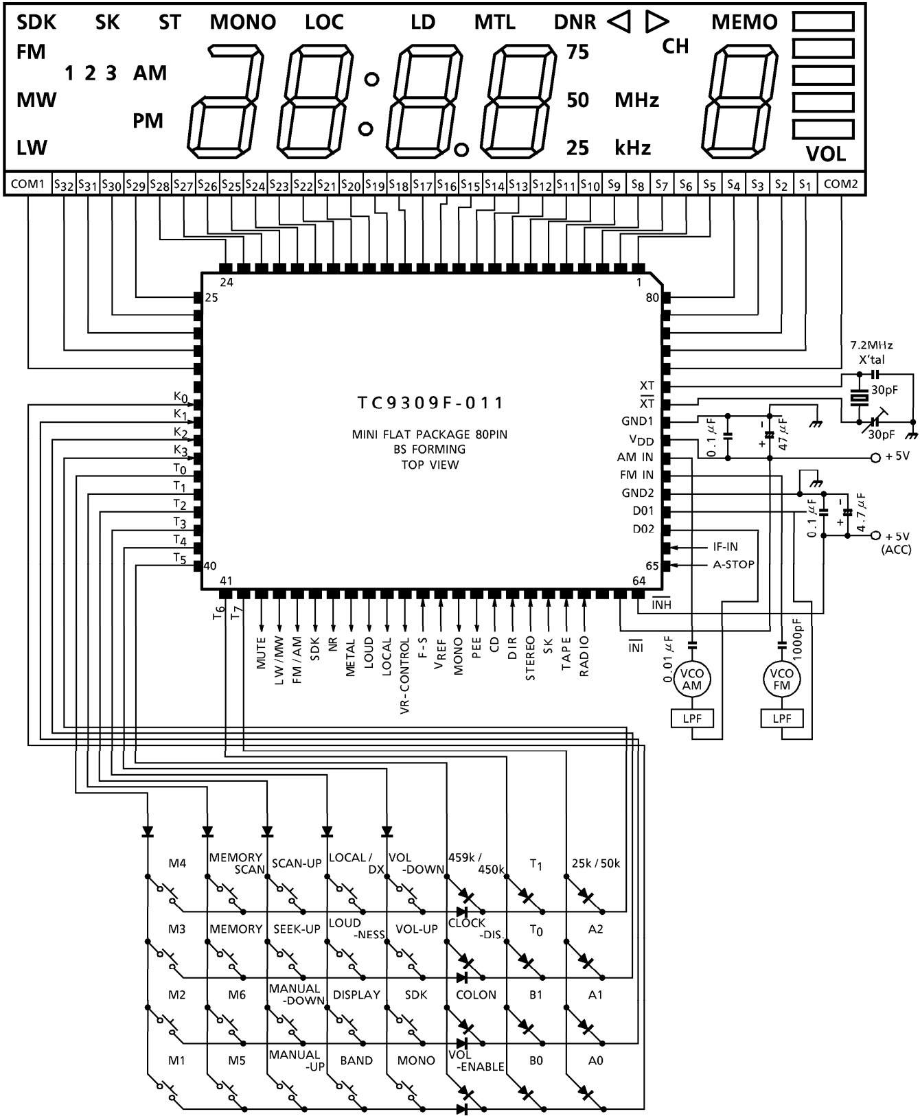
TC9309F-011 Layout
