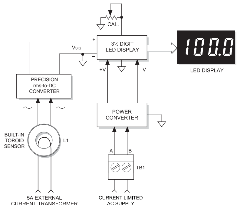
Figure 1. ACA5-20RM Series simplified schematic
