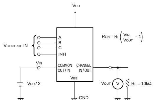
Fig. 2 ON resistance
