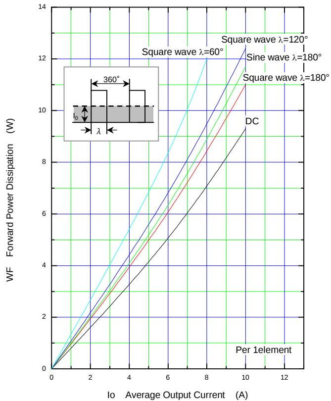
Forward Power Dissipation (max.)
