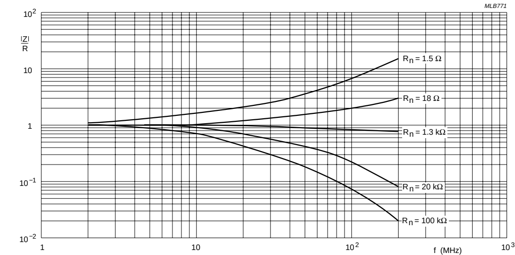
Fig.38 Impedance as a function of applied frequency.
