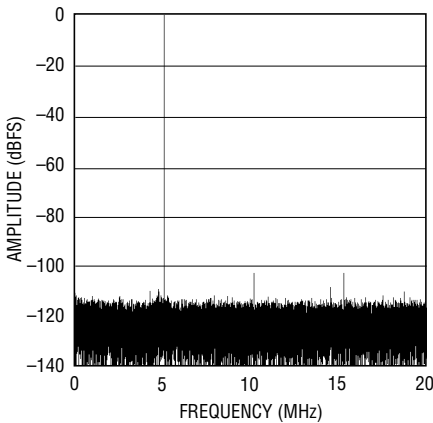
LTC2204: 64K Point FFT, 40Msps, f_{IN} = 5.1\text{MHz} , -25dBFS, PGA = 1, DITH = 0
