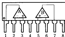
NJM2100L
