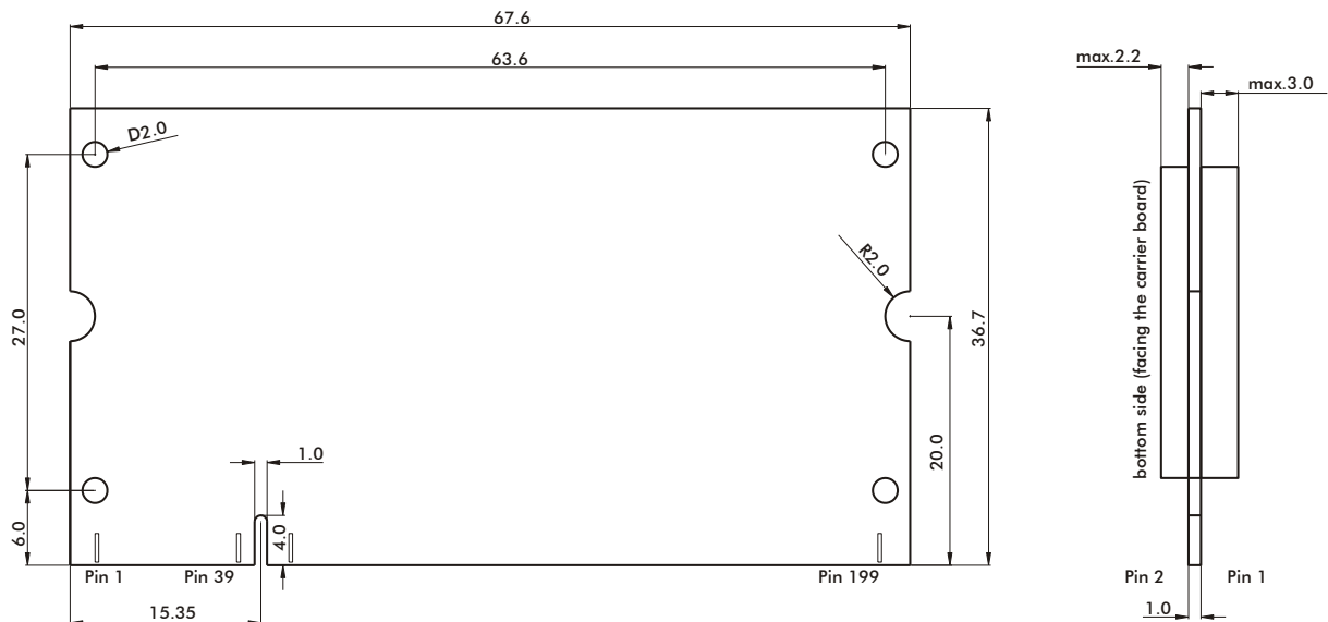
Figure 3: Mechanical dimensions of the Colibri PXA320 module
