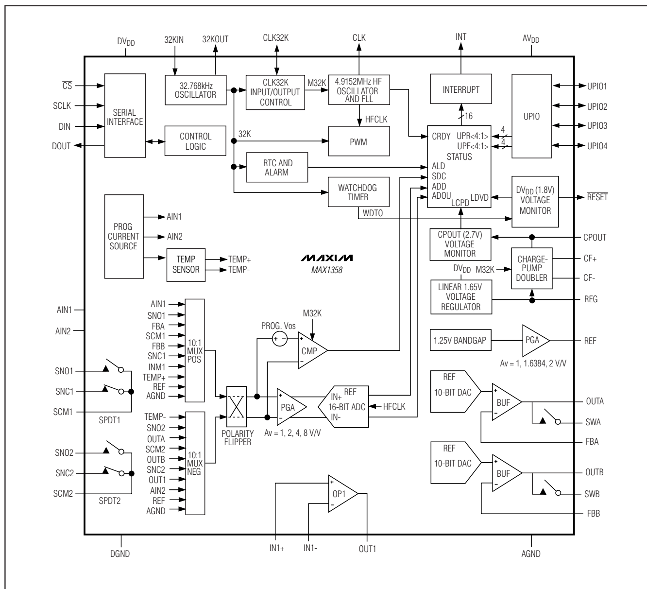
Figure 3. MAX1358 Functional Diagram
