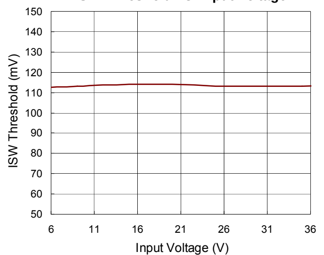
ISW Threshold vs. Input Voltage
