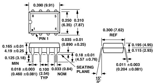
CERDIP (Q-8)
