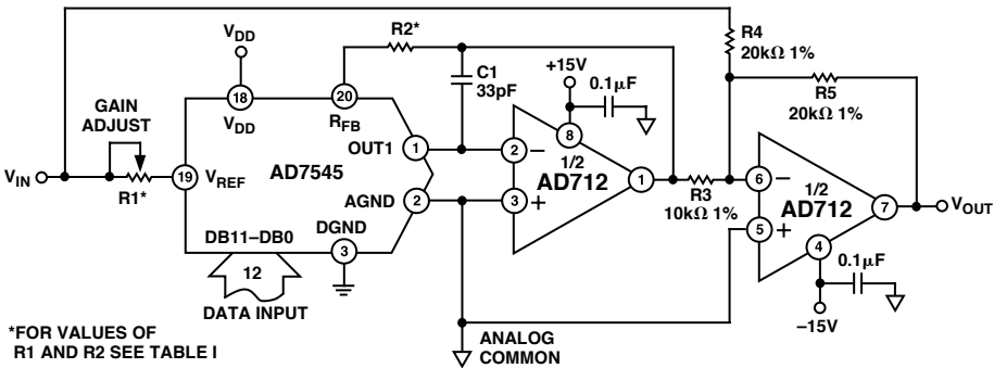
Figure 9. Bipolar Operation
