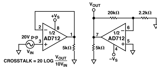
TPC 21. Crosstalk Test Circuit
