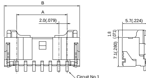
(10 to 12 circuits)
