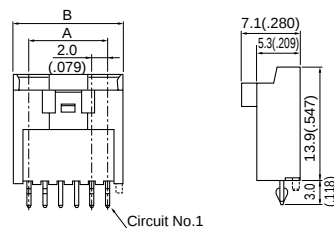
(5, 6 circuits)
