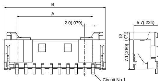
(10 to 12 circuits)
