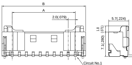
(10 to 13 circuits)
