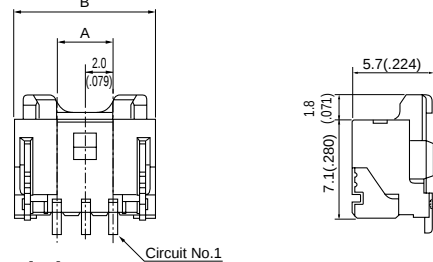
(4 to 9 circuits)
