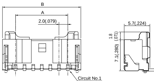
(10 to 13 circuits)
