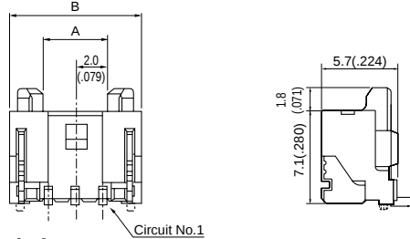
(4 to 9 circuits)
