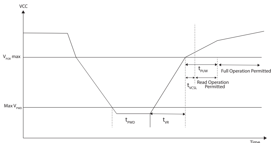
Figure 16-1. Power-Up Timing
