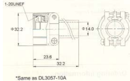
Cable Clamp
