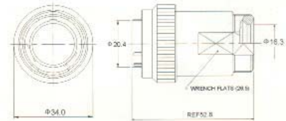
Straight Plug
