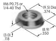
AT536 Hex Nut Nickel/brass Series: FB
