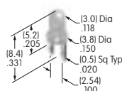
AT633 Single Element LED Colors: C D F Series: HB T-1 Bi-pin
