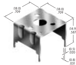
AT543 Support Bracket Tin/steel Series: MR
