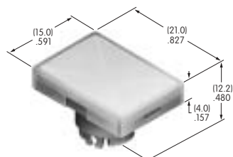
AT3016 Rectangular Cap for Super Bright LED Polycarbonate Colors: JB Series: YB
