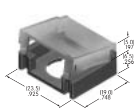
AT4028 Rectangular Cap for LED Polycarbonate Colors: JB JC JD JF Series: LB
