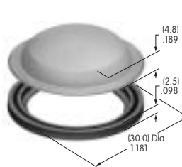
AT4013 Round Colored Insert Cap Polycarbonate Colors: JB JC JE JF JG Series: LB
