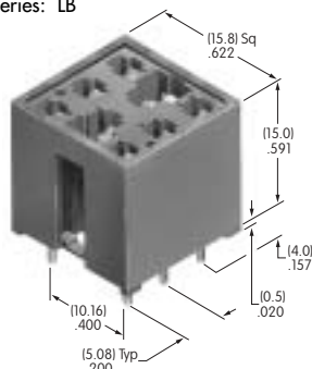
AT712 Double Pole Straight PC Adaptor Glass fiber reinforced polyamide Series: LB
