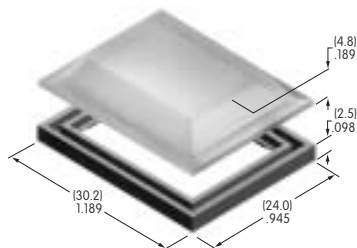
AT4011 Rectangular Splash Cover Polyvinyl chloride & polyethylene Series: LB UB
