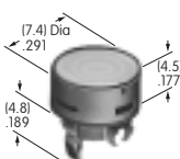
AT4032 Round Cap for Bright & Super Bright LED Polycarbonate Colors: JB Series: HB
