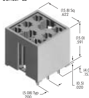
AT711 Single Pole Straight PC Adaptor Glass fiber reinforced polyamide Series: LB
