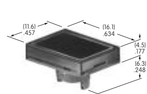
AT4022 Rectangular Colored Insert Cap Polycarbonate Colors: JB JC JE JF JG Series: KB
