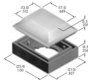
AT4030 Rectangular Nonilluminated Cap Polycarbonate Colors: A B C E F G H Series: LB
