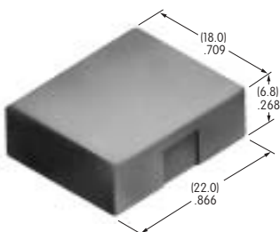
AT3076 Flat Cap for Illuminated with Lens/Diffuser Polycarbonate Colors: JB JC JD JF Series: UB2
