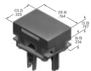
AT4031 Square Cap for Bright & Super Bright LED Polycarbonate Colors: JB Series: HB
