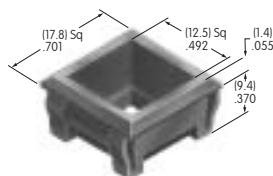
AT602 Incandescent Lamp Volts: 6 12 18 24 28 Series: LW MLW T-1 1/2 Pilot Slide Base
