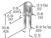
AT631 Single Element LED Color: B Series: KB LB YB T-1 Bi-pin
