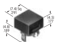
AT4035 Square Nonilluminated Cap Polycarbonate Colors: A B C E F G Series: HB
