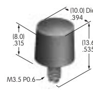
AT092 Knurled Mounting Nut Polyphenylene oxide Series: YB
