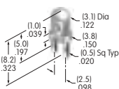
AT630 Single Element LED Color: F Series: HB T-1 Bi-pin
