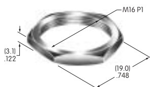
AT056 Dress Cap Nut Chrome/brass Series: M P S
