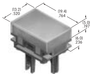
AT4033 Square Indicator Cap Polycarbonate Colors: JB Series: HB
