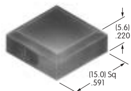
AT3075 Beveled Cap for Illuminated Polycarbonate Colors: B C D F Series: UB2
