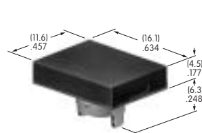
AT4021 Rectangular Solid Colored Cap Polycarbonate Colors: A BB CB CC EB FB FF GB GG Series: KB
