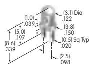
AT629 Single Element LED Color: B Series: HB T-1 Bi-pin
