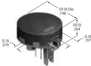
AT4016 Round Spot Illuminated Cap Polycarbonate Cap Colors: A B C F LED Colors: C D F CF Series: LB
