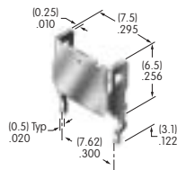
AT546 Mounting Bracket for Block Mounting Tin-lead/phosphor bronze Series: GB2
