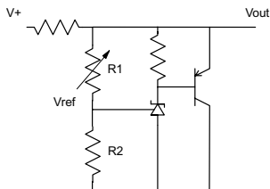
HIGHER CURRENT SHUNT REGULATOR
