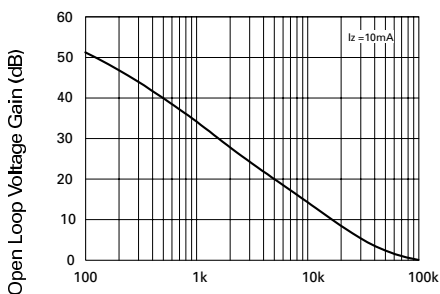
Gain v Frequency
