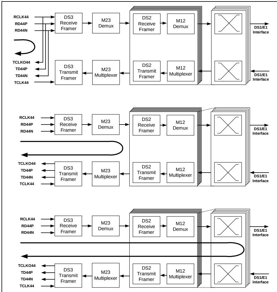
Figure 6 Remote Loops
