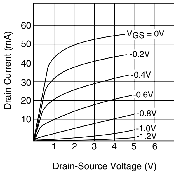
DRAIN CURRENT vs. DRAIN-SOURCE VOLTAGE
