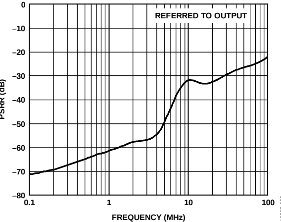
Figure 41. Power Supply Rejection Ratio (PSRR) vs. Frequency
