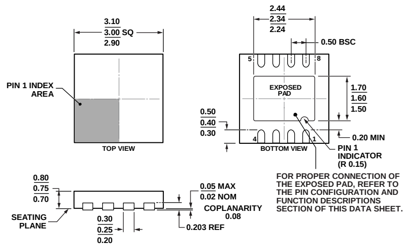
Figure 58. 8-Lead Lead Frame Chip Scale Package [LFCSP_WD] 3 mm × 3 mm Body, Very Very Thin, Dual Lead (CP-8-11)
