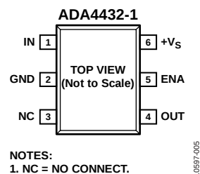
Figure 5. ADA4432-1 SOT-23 Pin Configuration, Top View
