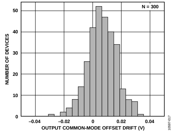
Figure 35. Total Output Common-Mode Offset Voltage Drift ( -40^{\circ}\text{C} to +125^{\circ}\text{C} )
