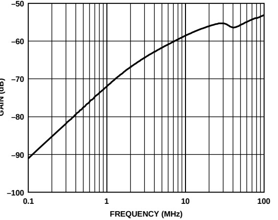
Figure 42. Input-to-Output Off (Disabled) Isolation vs. Frequency
