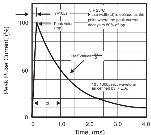
Fig.5 - Pulse Waveform
