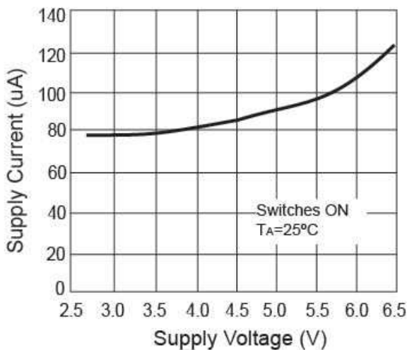
Figure 3. ON-State Current vs. Supply Voltage
