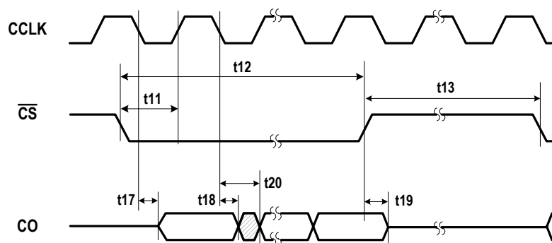
Figure - 8 MPI Output Timing
