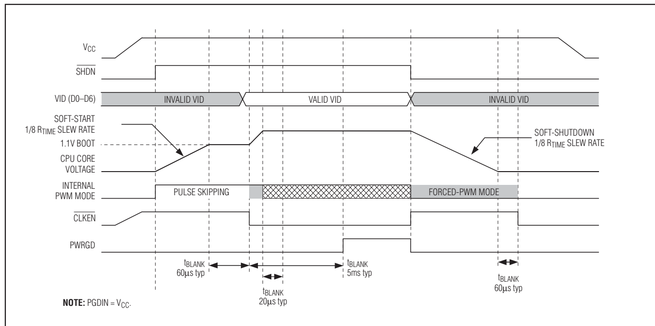
Figure 9. IMVP-6.5 Power-Up and Shutdown Sequence Timing Diagram
