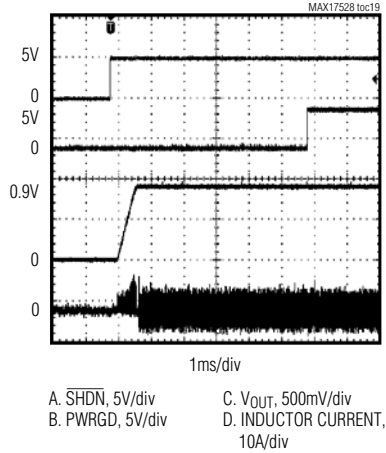
GMCH SOFT-START WAVEFORM
