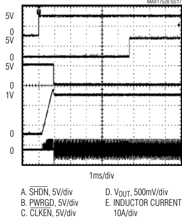
IMVP-6.5 SOFT-START WAVEFORM (UP TO PWRGD)
