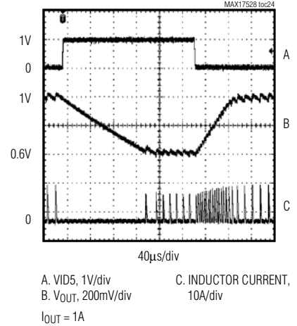
DPRSLPVR = HIGH, SLOW = LOW, VID5 TRANSITION
