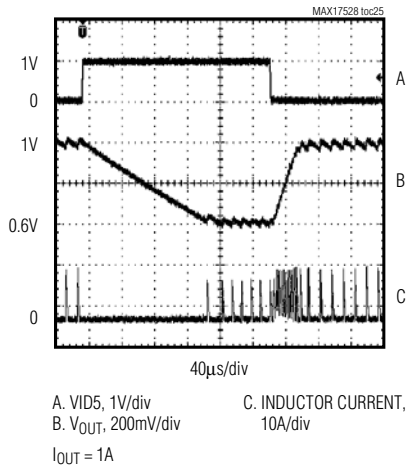
DPRSLPVR = HIGH, SLOW = HIGH, VID5 TRANSITION
