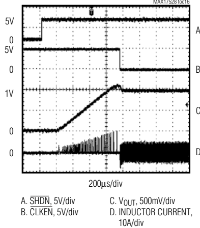
IMVP-6.5 SOFT-START WAVEFORM (UP TO CLKEN)
