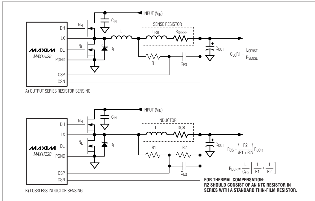
Figure 4. Current-Sense Methods
