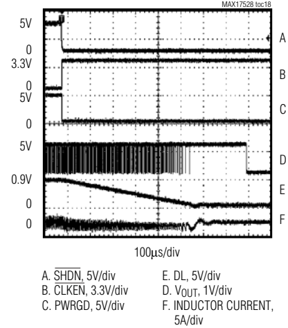
IMVP-6.5 SHUTDOWN WAVEFORM
