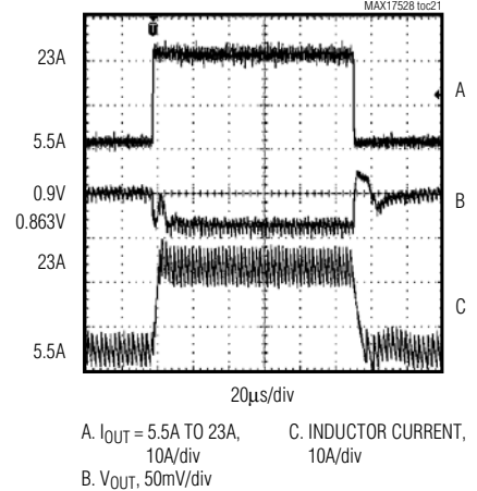
LOAD-TRANSIENT RESPONSE (IMVP-6.5 HFM MODE)
