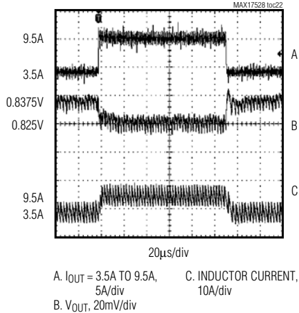
LOAD-TRANSIENT RESPONSE (IMVP-6.5 LFM MODE)
